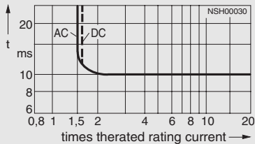
Characteristic curve of short-circuit releases
