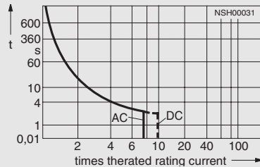
Characteristic curve of combined overload and short-circuit releases at an ambient temperature of 40 °C
