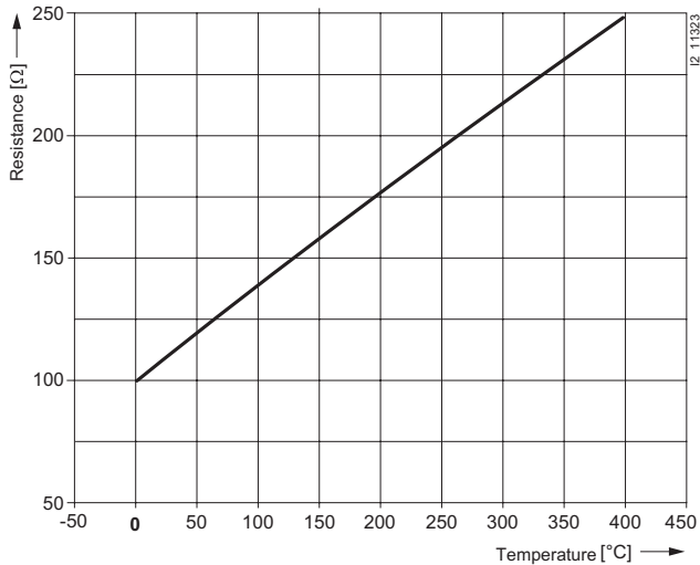
Resistor characteristic curves PT100 according to EN 60751 (96)
