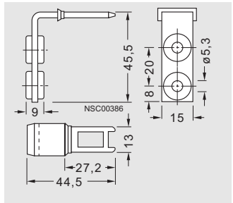
3SX3 253 actuator with vertical fixing
