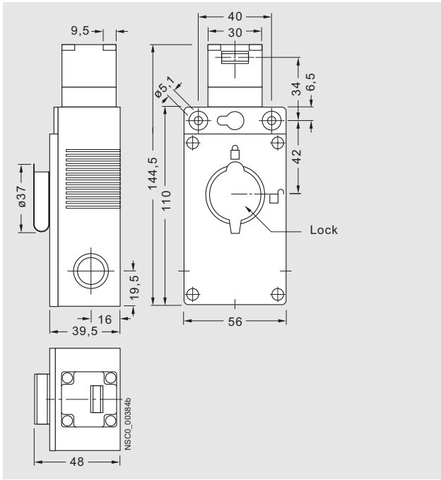
3SE3 75.-XX, 3SE3 76.-XX molded-plastic enclosures
