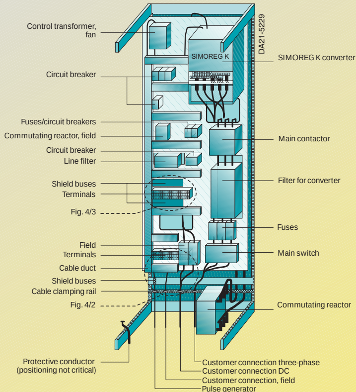
Fig. 4/1 Example of cabinet arrangement with a SIMOREG K
